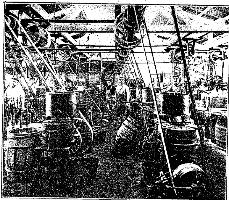
Grinding Department. A Well Room
